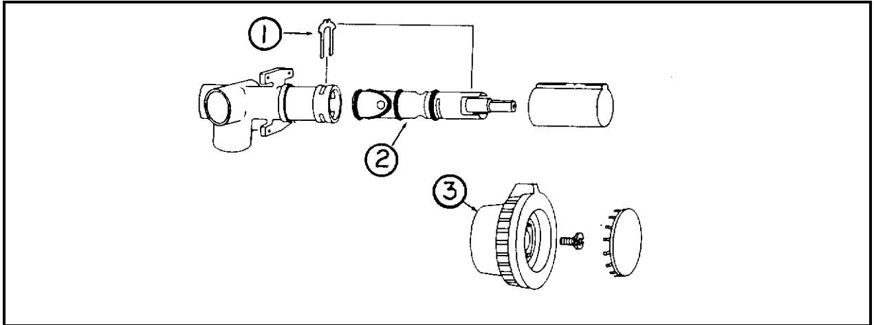
601420-01Faucet, shower
