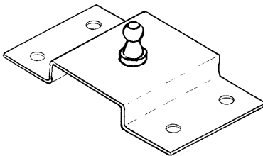
381673 Prop bracket, raised, jamb mount
