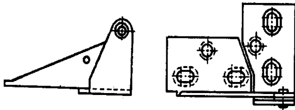
385935 Hinge, pivot, brass for bath mirror
