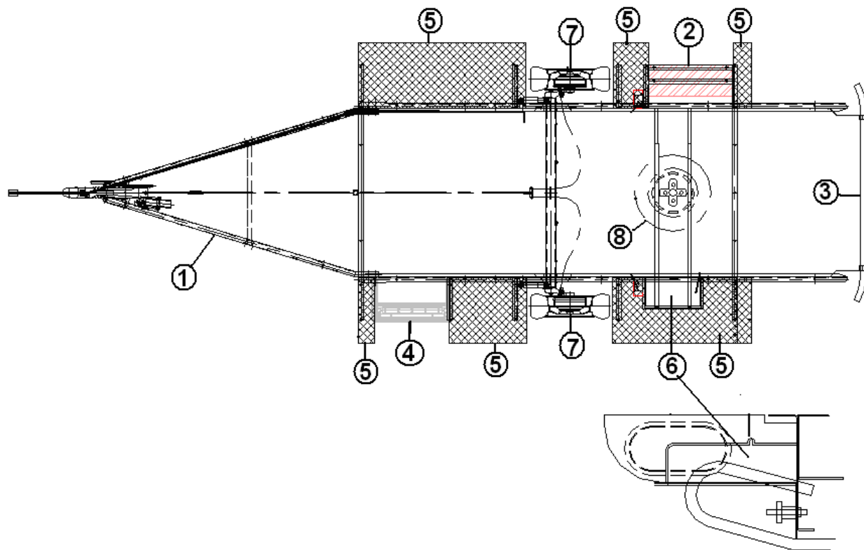
Chassis Diagram, 532
