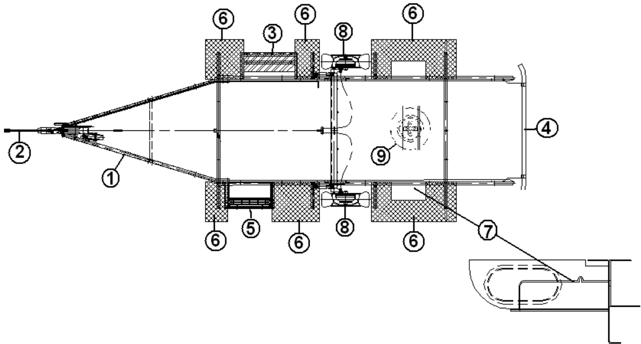
Chassis Diagram, 534 AEU
