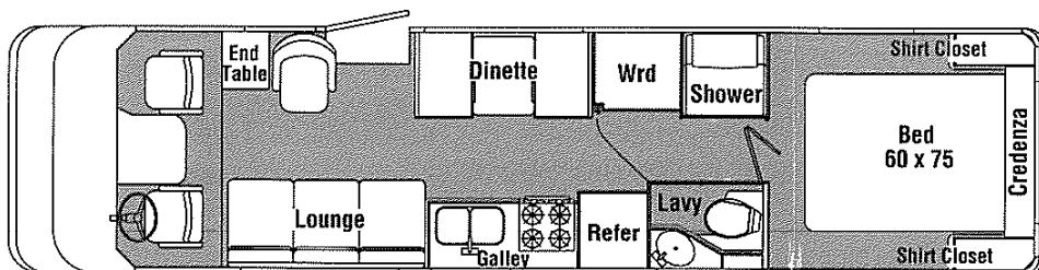
33' LAND YACHT
