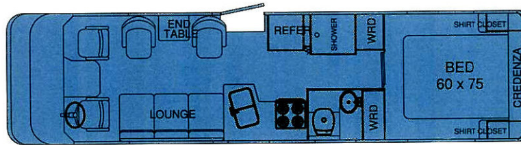
30' LAND YACHT
