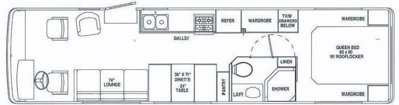
34' Cutter
