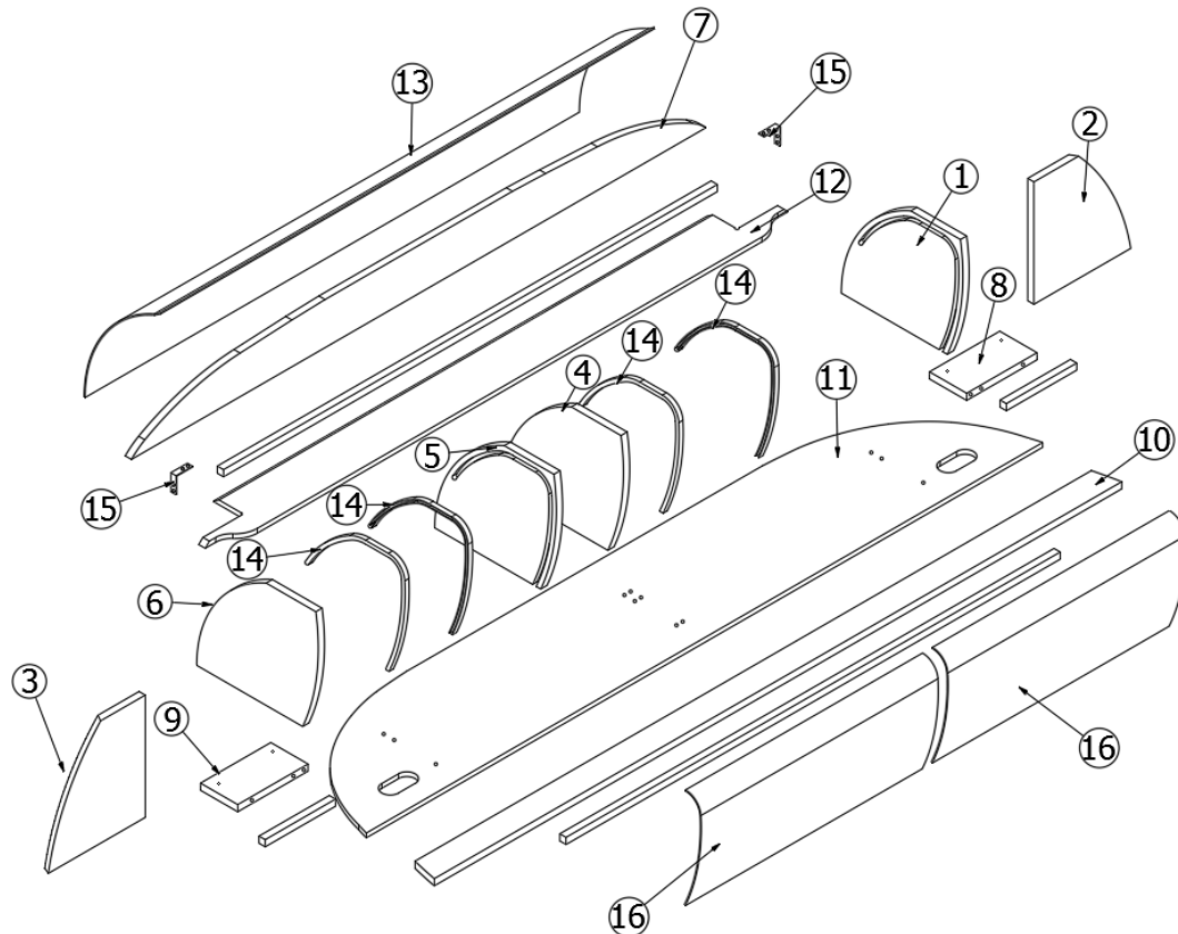
969098 Ass'y, Front Liner Locker
