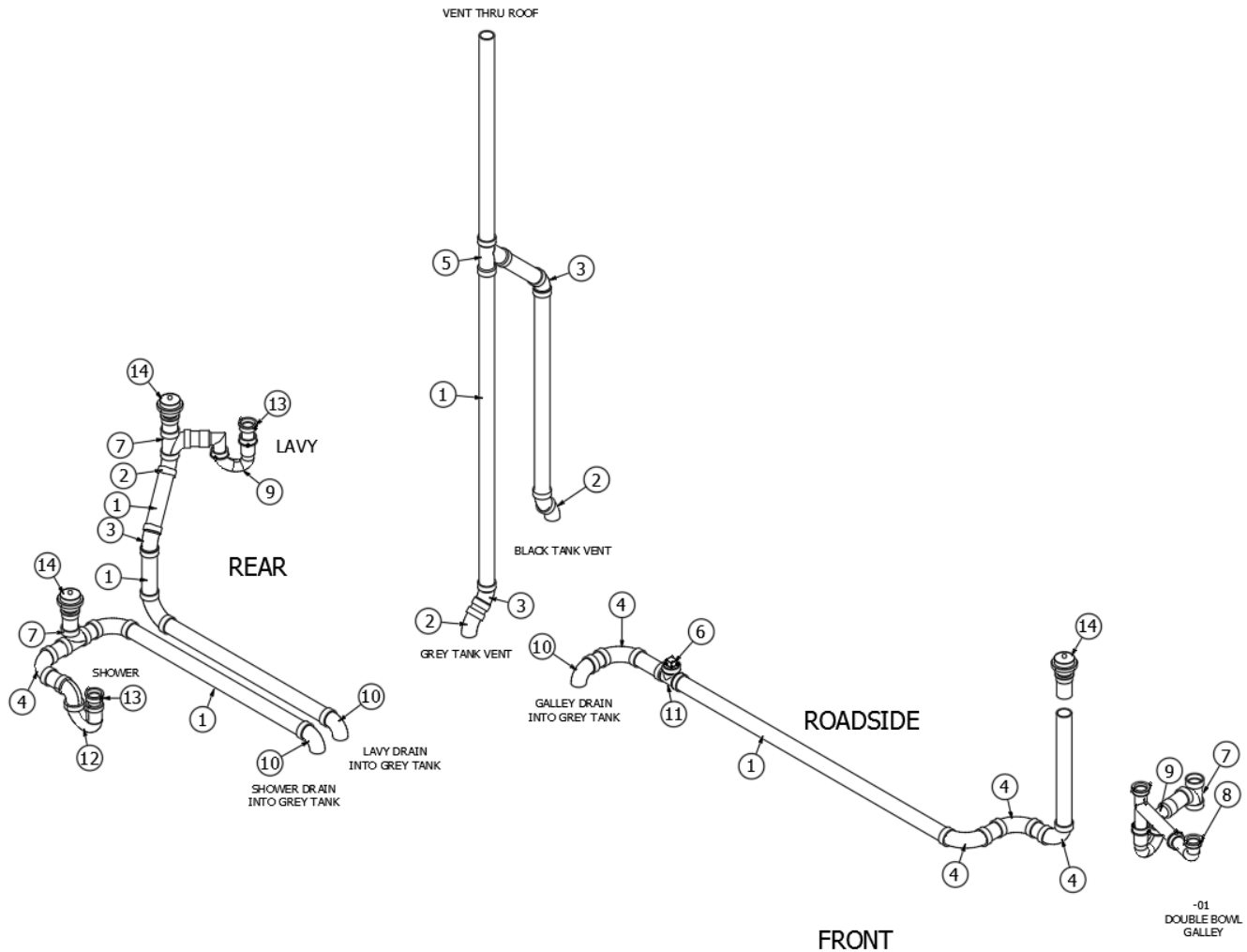
943900-01 Layout - Above Floor Drain 22' Bambi
