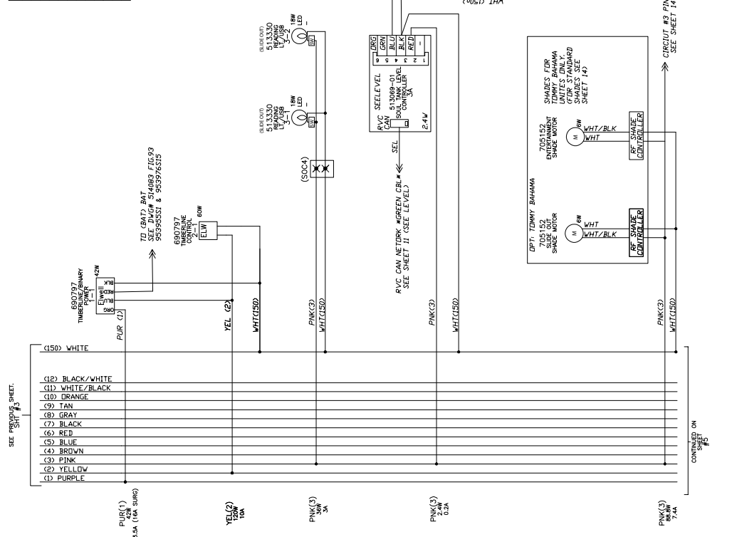
CIRCUIT CIRCUIT WATTS AMPS @ 12VDC CIRCUIT FUSE (AMP) PURPLE (1) 42 3.5 (16A Spike) 20 PURPLE (2) 122.60 10.45 15 PINK (1) 10.75 0.9 15 PINK (2) 17.75 1.5 15 BROWN (4) 157.5 9.6 15 BLUE (3) 131.88 10.99 15 RED (1) 120 10 15 RED (2) 190.68 15.89 20 RED (3) 160 15 15 TAN (3) — — — ORANGE (10) — — — WHITE/BLACK (1) 286 24 30 BLACK/WHITE (2) 153.96 12.66 15
