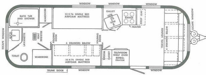
TWIN BED
