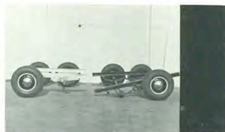
Dura-Torque axle (left) shows Airstream's perfect suspension. Drive on any three wheels for miles!
